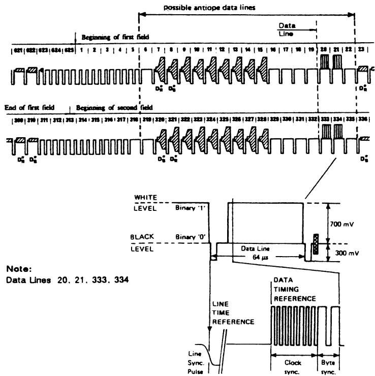
Fig. 3 Identification and Levels of Antiope Data Lines
