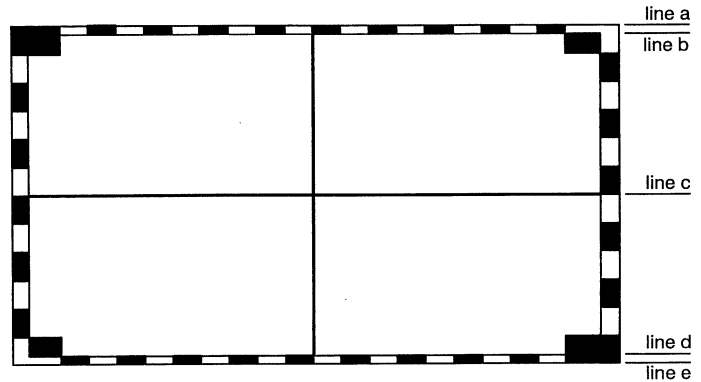
Fig. 5 Center Cross; 625 / 525 Lines; Aspect Ratio 16:9
